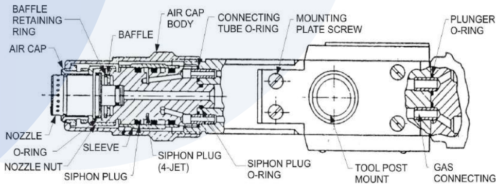
FIGURE 8.2 TYPE 6PM-II BOTTOM VIEW
