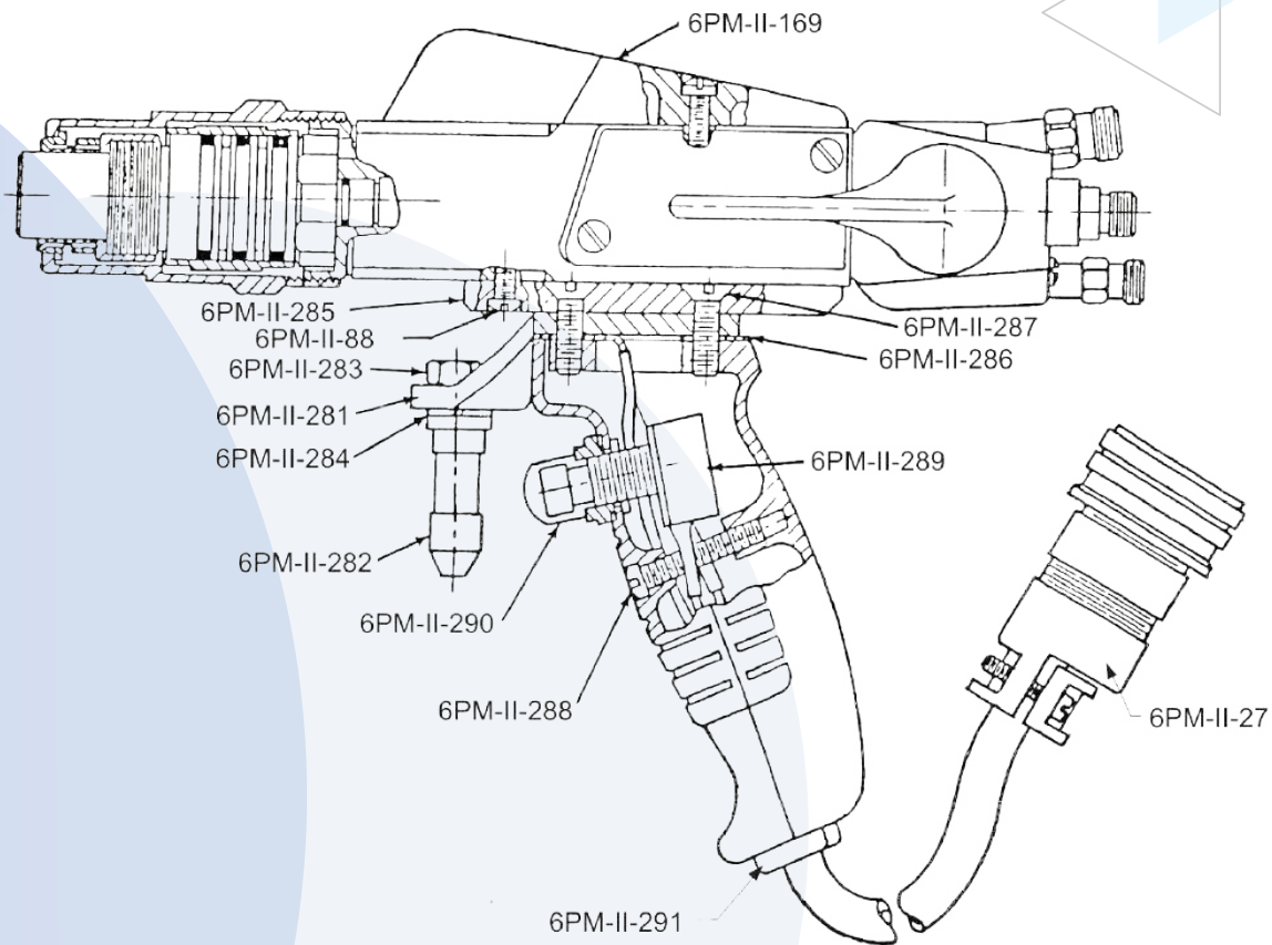
FIGURE 10.3 TYPE 6PM II-H POWDER FLAME SPRAY GUN FOR HAND-HELD MANUAL OPERATION
