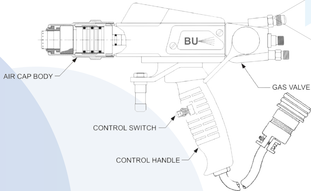
FIGURE 1.2 TYPE6PM-II-H HAND-HELD POWDER FLAME SPRAY GUN
