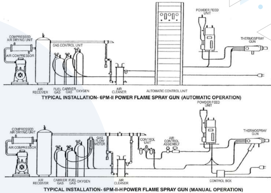
FIGURE 5.1 TYPICAL POWDER FLAME SPRAY SYSTEM INSTALLATION
