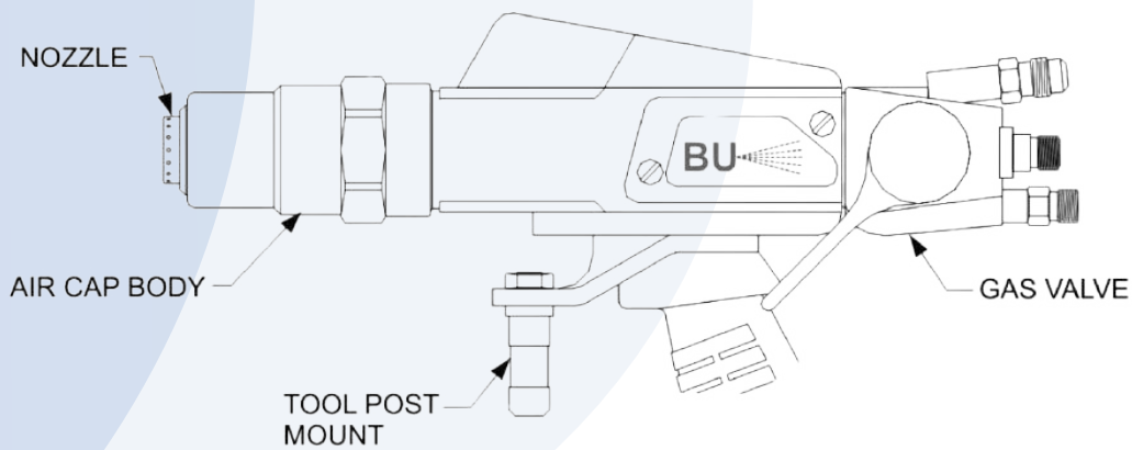
FIGURE 1.3 TYPE 6PM- II-A AUTOMATIC POWDER FLAME SPRAY GUN
