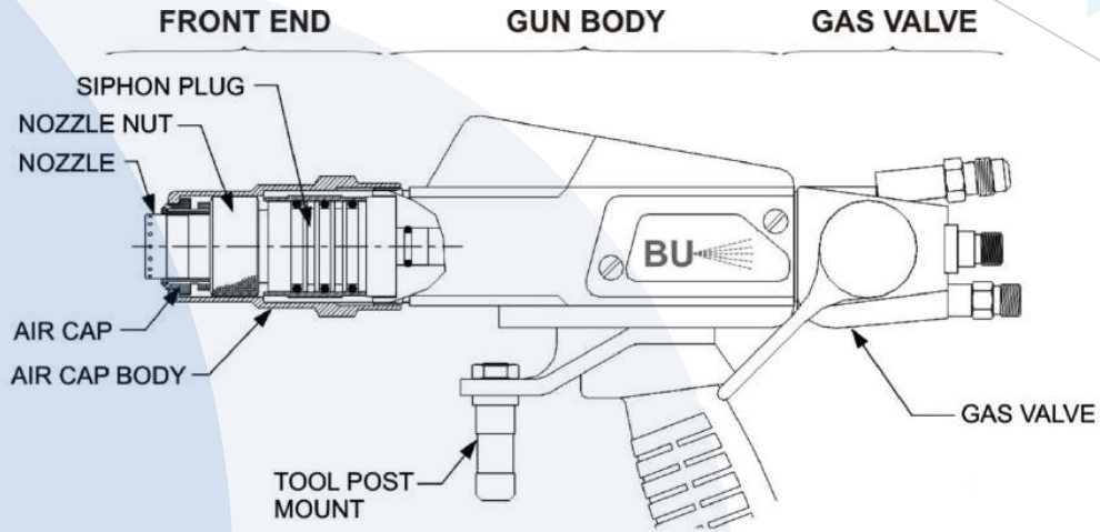
FIGURE 8.1 TYPE 6PM-II POWDER FLAME SPRAY GUN
