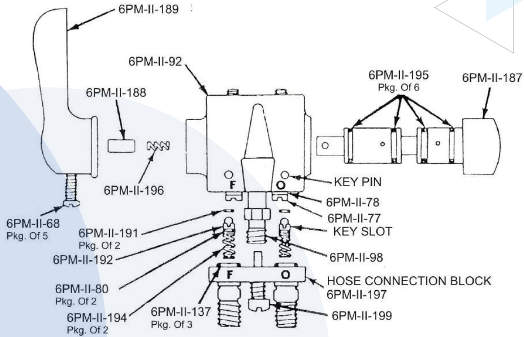
TYPE 6PM -II-H POWDER FLAME SPRAY GUN
