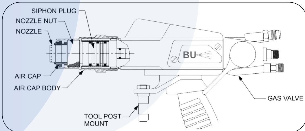
FIGURE 1.1 TYPE 6PM -II POWDER FLAME SPRAY GUN
